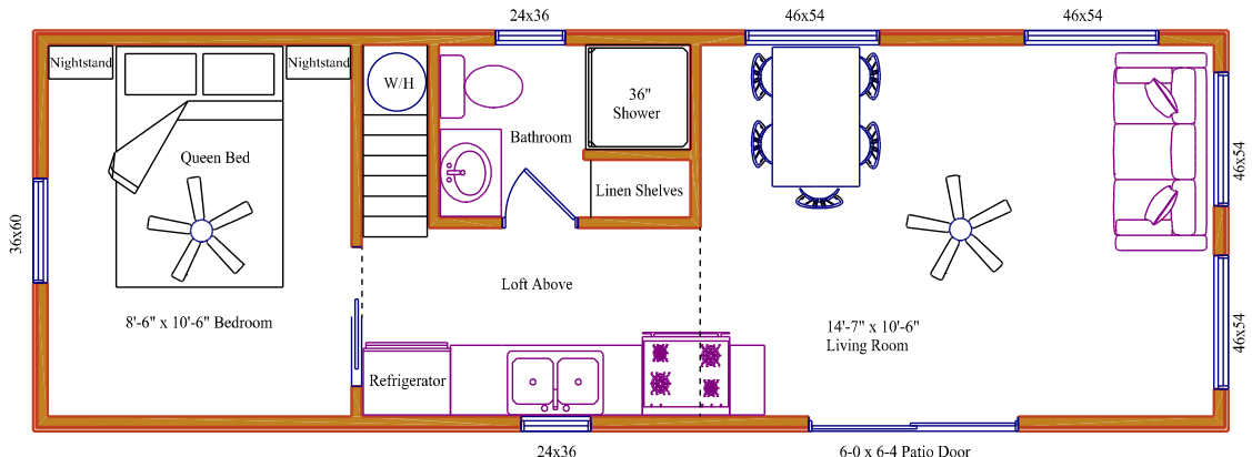
Model P34 – Size: 11'-3" x 34', 1 Bedroom, Loft
