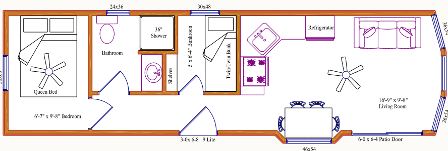
Model L37 – Size: 10'-5" x 37', 2 Bedroom, Bay Window
