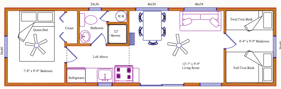
Model P37 – Size: 10'-6" x 37', 2 Bedroom, Loft
