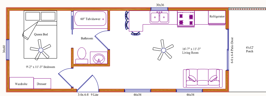
Model L38 – Size: 12' x 32', 1 Bedroom with 6' porch
