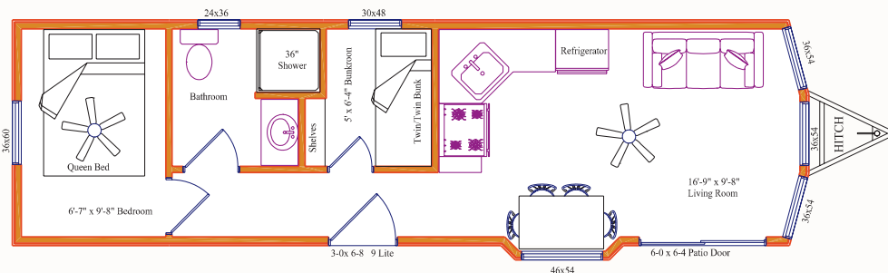
Model L37 - Size: 10'-5" x 37', 2 Bedroom, Bay Window
