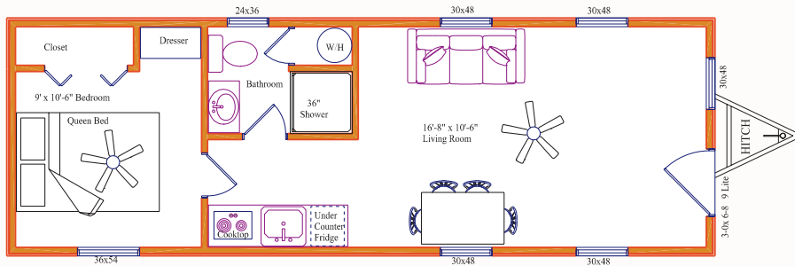
Model L34 - Size: 11'-3" x 34', 1 Bedroom
