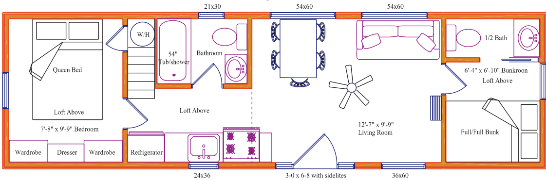
Model K37 - Size: 10'-6" x 37', 2 Bedroom, 1-½ Bath, Double Loft
