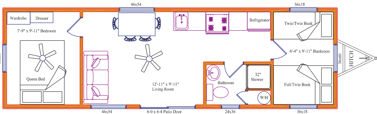
Model L36 - Size: 10'-8" x 36', 2 Bedroom
