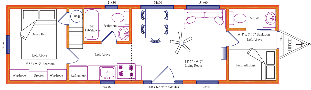
Model K37 – Size: 10'-6" x 37', 2 Bedroom, 1-½ Bath, Double Loft
