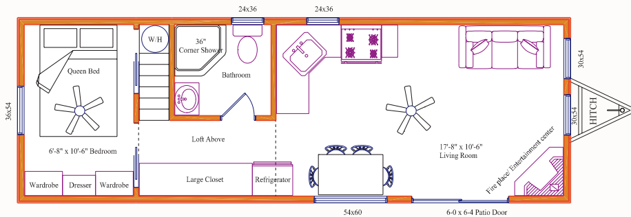
Model K34 – Size: 11'-3" x 34', 1 Bedroom, Loft
